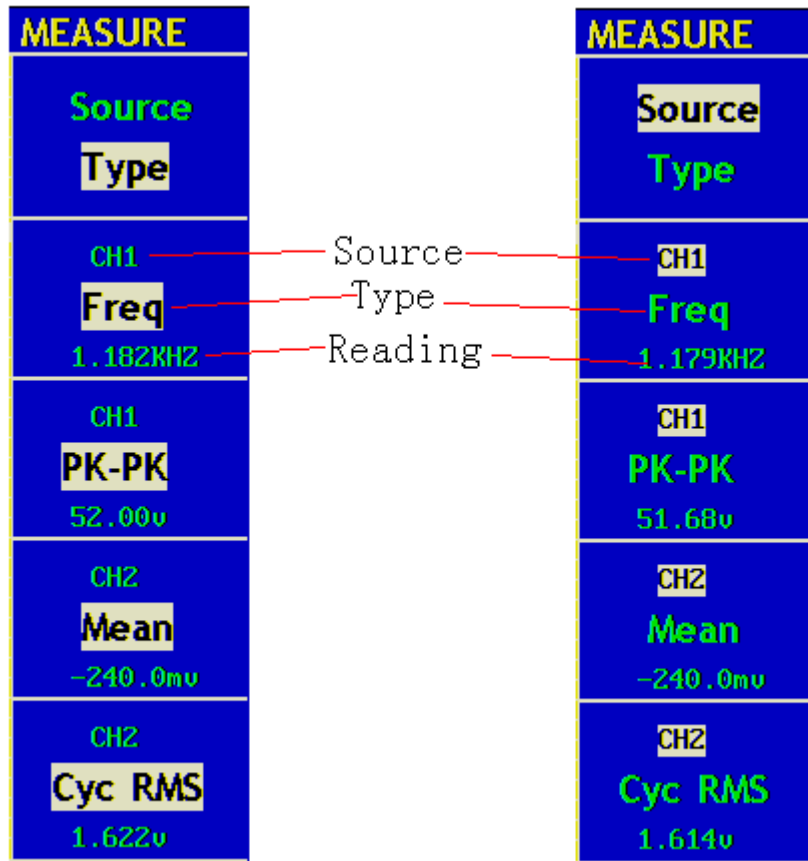
Fig. 48 Measure Menu
