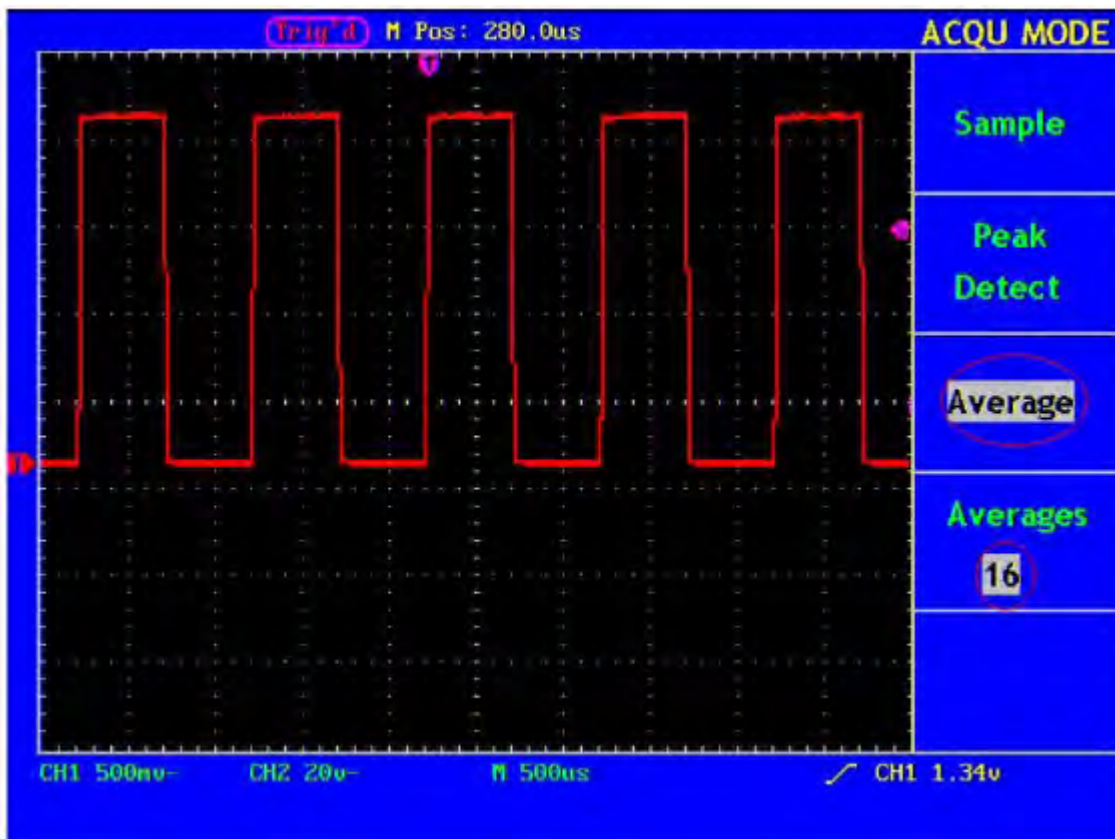
Fig. 36 The displayed wave form after the noise is removed under the Average Mode, in which the average number of 16 is set.
