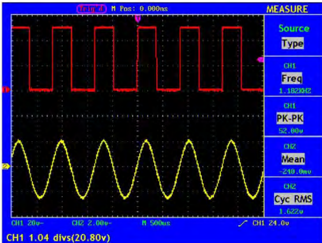
Fig. 49 Automatic Measurement
