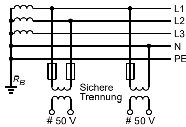
Abb. 22: SELV
